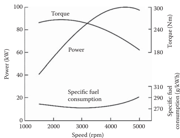
FIGURE 4.3 Typical performance characteristics of gasoline engines.
